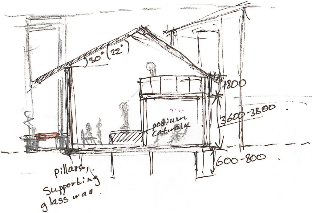
Section of the building (A-A)
